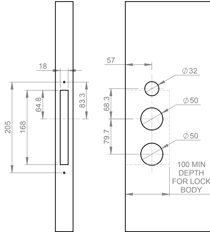
TYPICAL ALUMINIUM DOOR ROUTING
