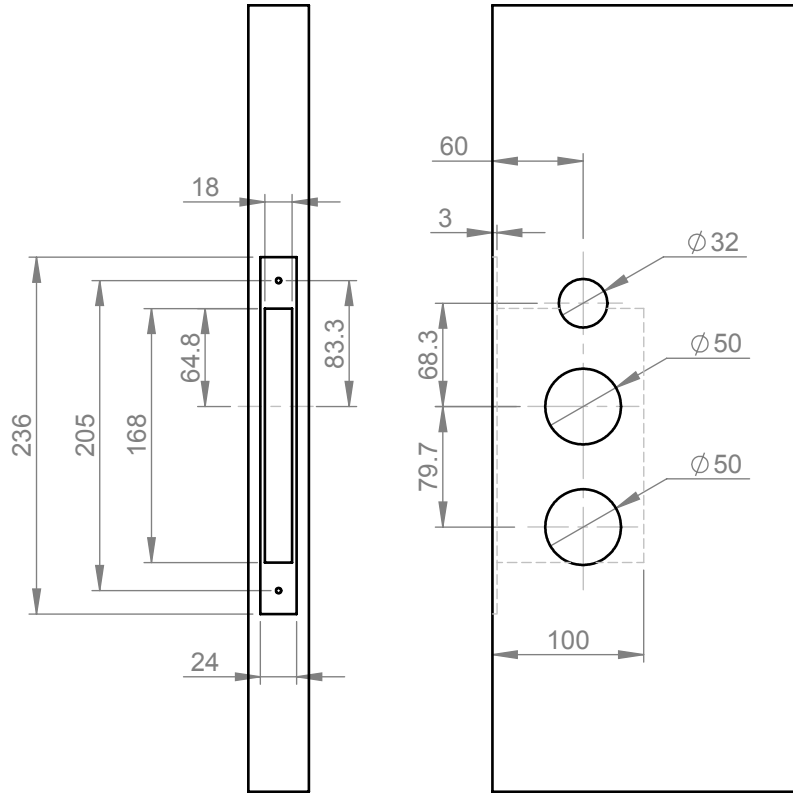
TYPICAL WOODEN DOOR ROUTING
