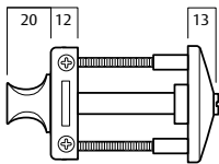
Toilet bolt with indicator (emergency release)
