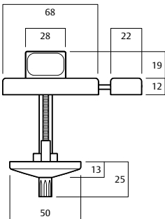
Toilet bolt with indicator (hospital release)
