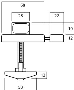
Toilet bolt with indicator (emergency release)
