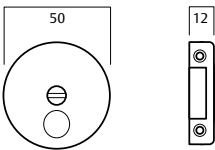
Toilet bolt with indicator (hospital release)
