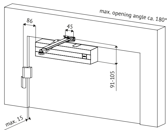
OPENING SIDE
