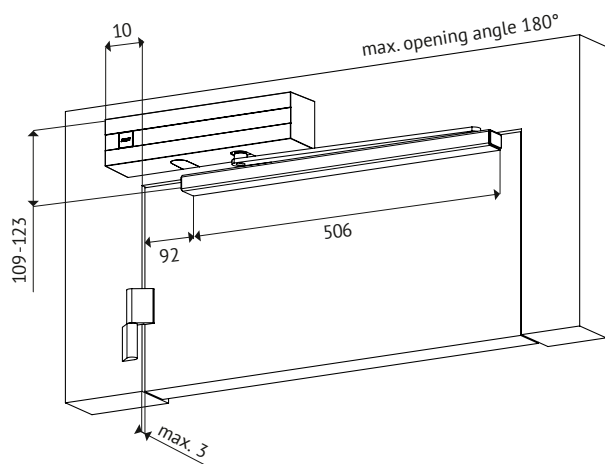
CLOSING SIDE
